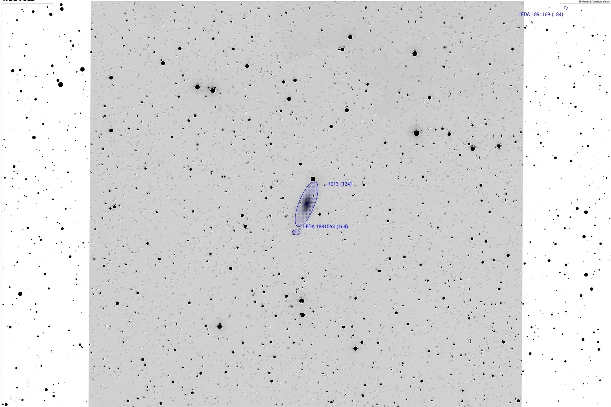
NGC 7013 (Galaxy) aka MCG 5-49-1, UGC 11670, Z 491-2, H II-203, PGC 66003 Magnitude: 12.40 B Size: 4.2' x 1.4' Sa, Nearly edge on SBr: 22.4 Mag/arcsec 2
