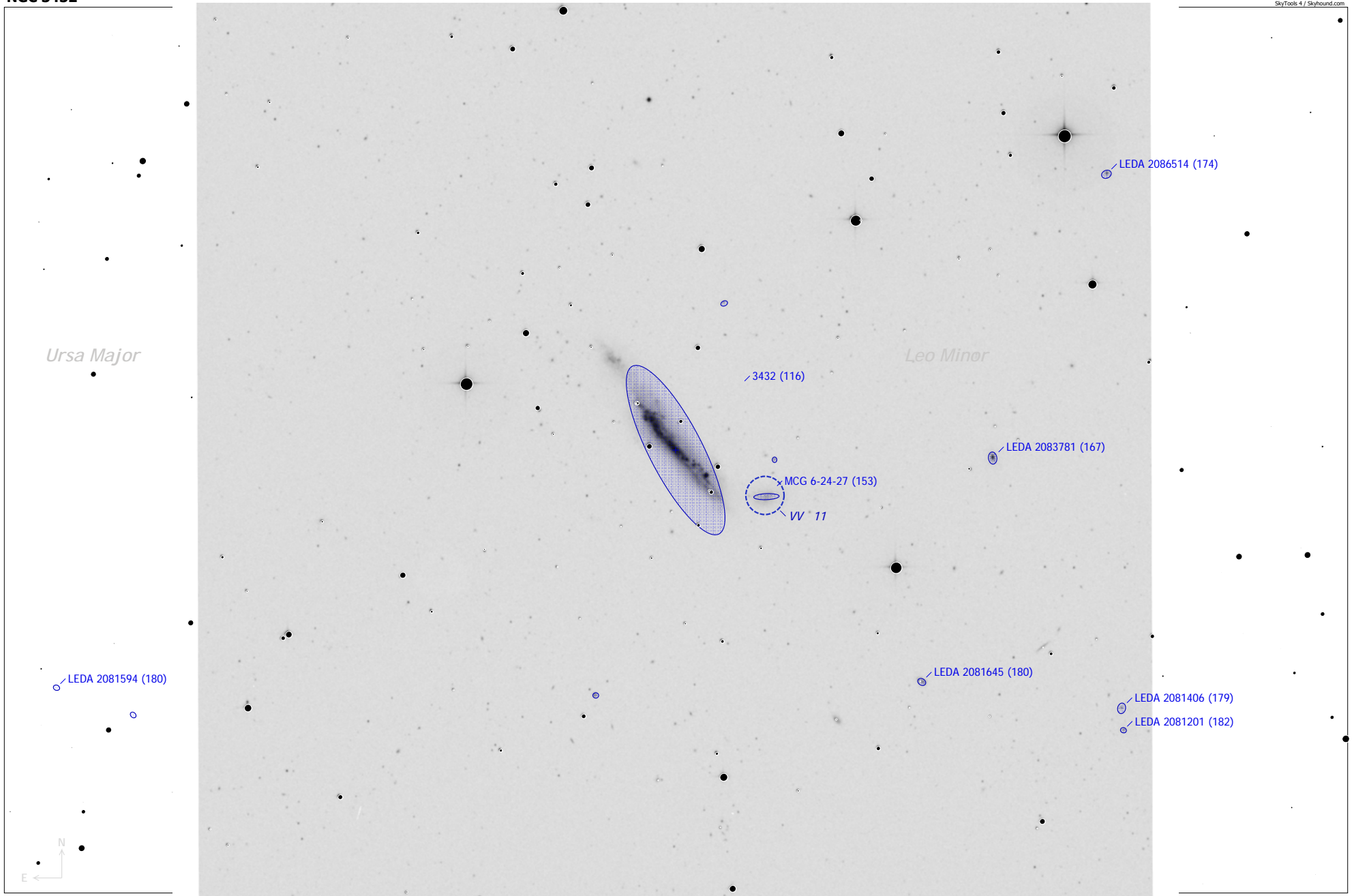
NGC 3432 (Galaxy) aka Arp 206, MCG 6-24-28, UGC 5986, Z 184-30, H I-172, PGC 32643 Magnitude: 11.60 B Size: 7.4' x 2.1' SBm, Nearly edge on SB: 22.7 Mag/arcsec 2
